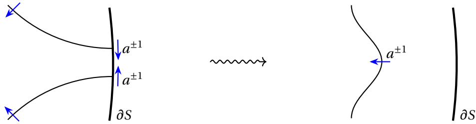
Figure 3: Splicing adjacent endpoints (Move 3)
