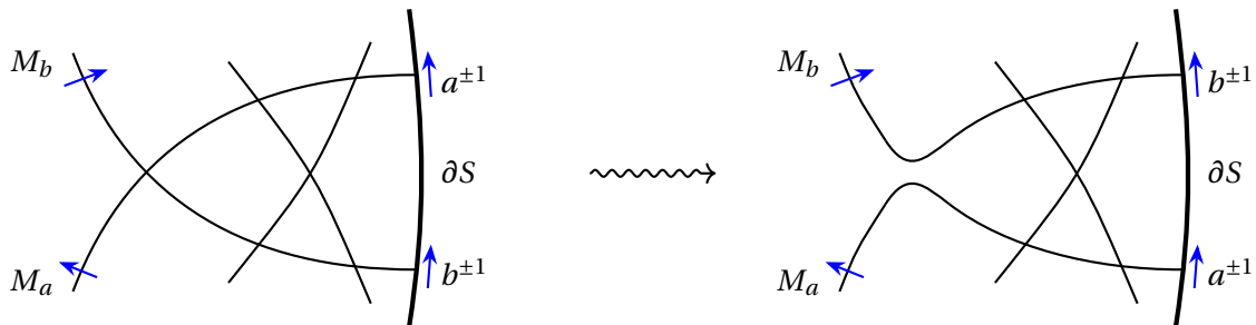
Figure 2: Removing an innermost half-bigon (Move 2)
