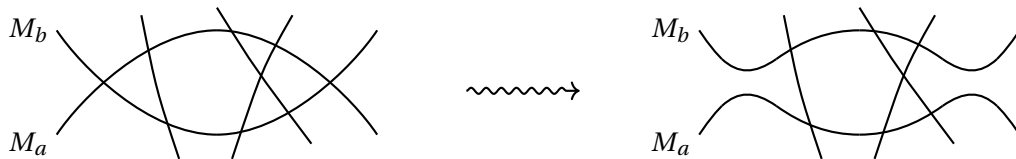
Figure 1: Removing an innermost bigon (Move 1)
